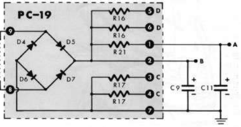
SCHMATIC DIAGRAM
